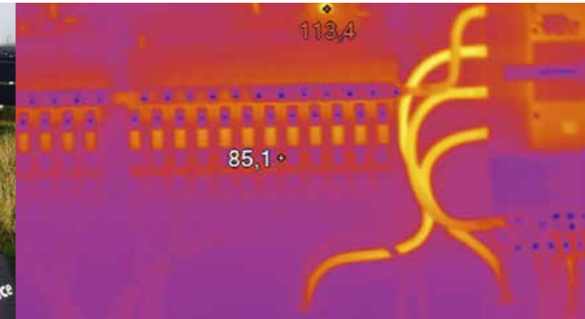
When commissioning a solar farm, all DC sub-distributors are inspected by GP JOULE using a thermal-imaging camera.
